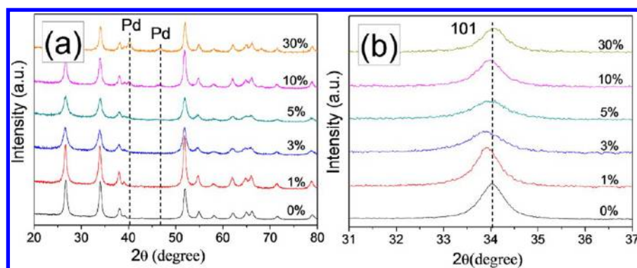
Figure 4. (a) Full-angle range of XRD patterns of pristine and Pd 0 -loaded SnO 2 nanofibers. (b) High-resolution of (101) peak.
