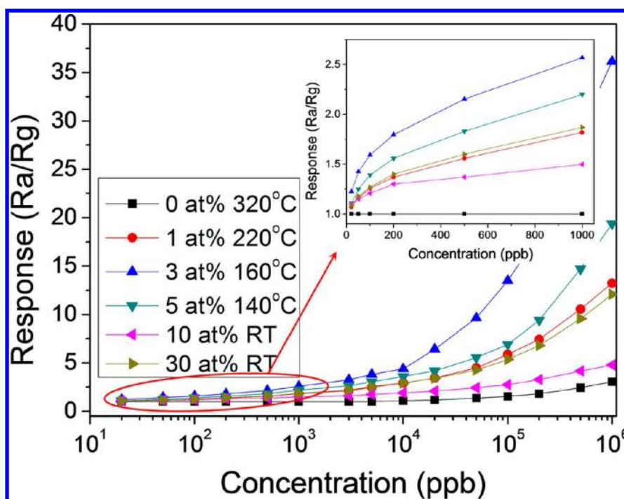
Figure 7. Linear plots of the response of the sensors based on Pd 0 -loaded SnO 2 nanofiber against H 2 in the range of 20 ppb to 1000 ppm at different operating temperatures. The inset presents the acceptable response of them at low H 2 concentration.
